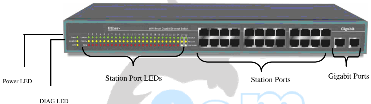
Fig. 2-2 Front Panel
