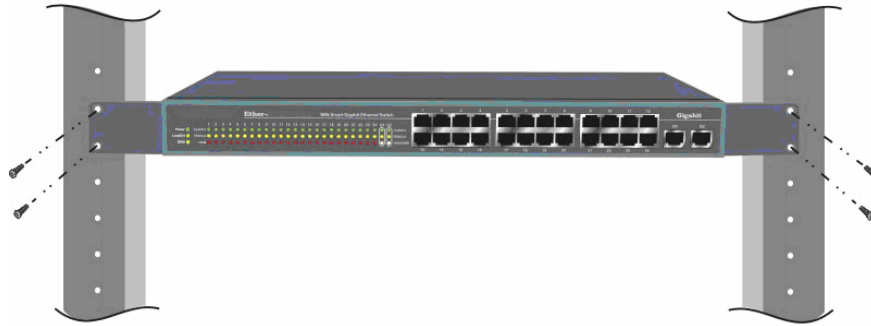
Fig. 3-2 Attaching the Switch to a 19-inch rack
