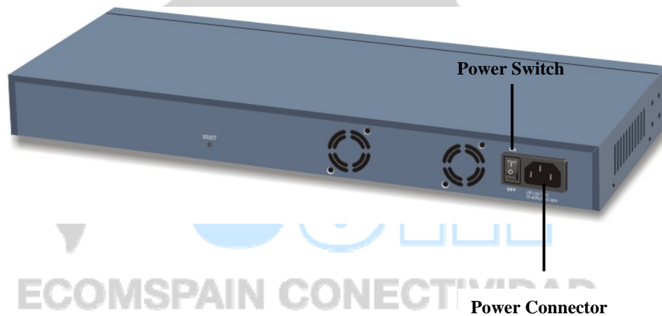
Fig. 2-4 Rear Panel
