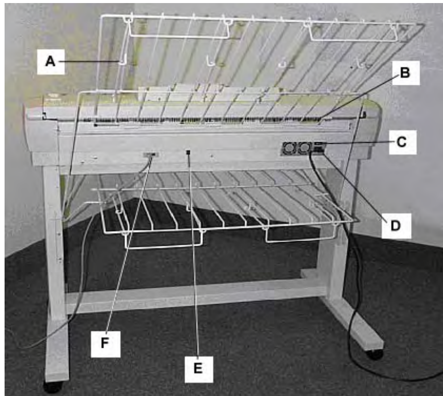
WIDE FORMAT SCAN SYSTEM Rear View
