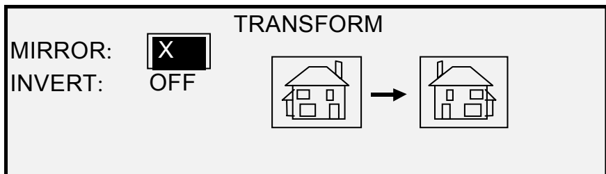
Transform Screen
