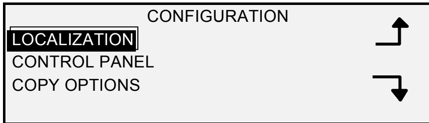
Configuration Screen
