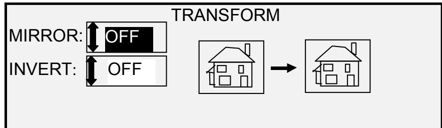
Transform Screen
