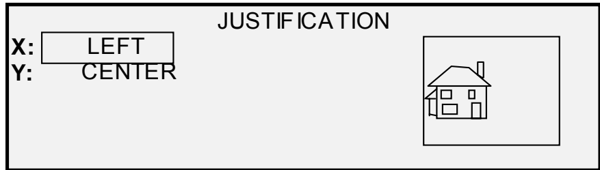
Justification Screen
