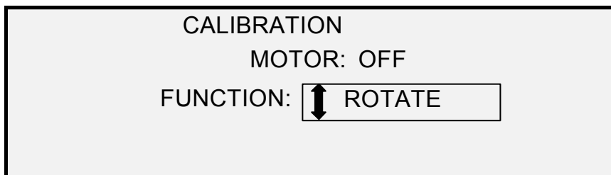
Calibration Screen
