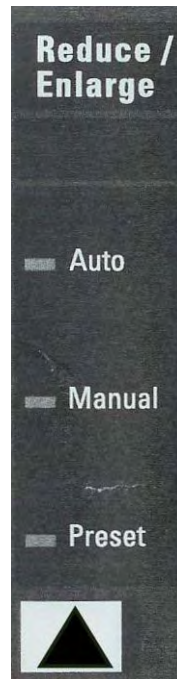
Reduce/Enlarge Area
