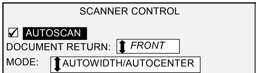
ScannerControl Screen
