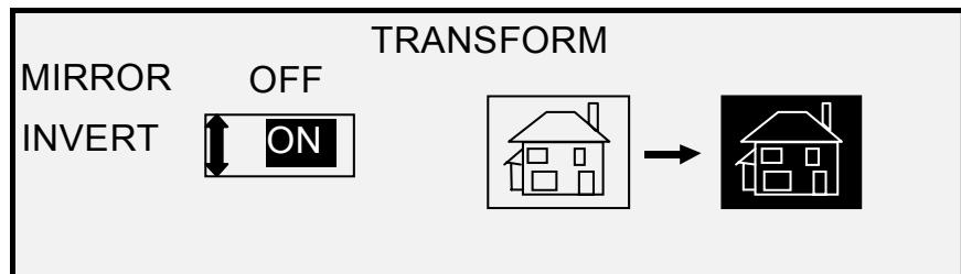
Transform Screen
