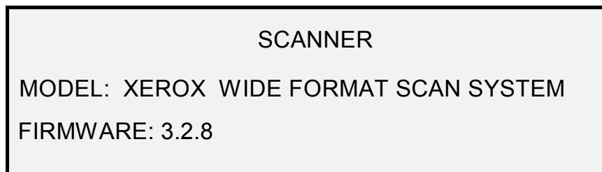
Scanner Screen
