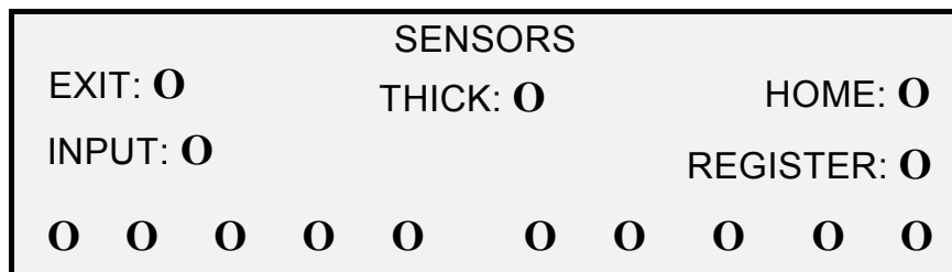
Sensors Screen
