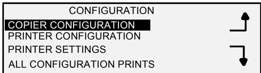
Configuration Screen
