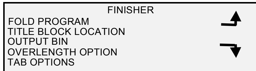
Finisher Screen
