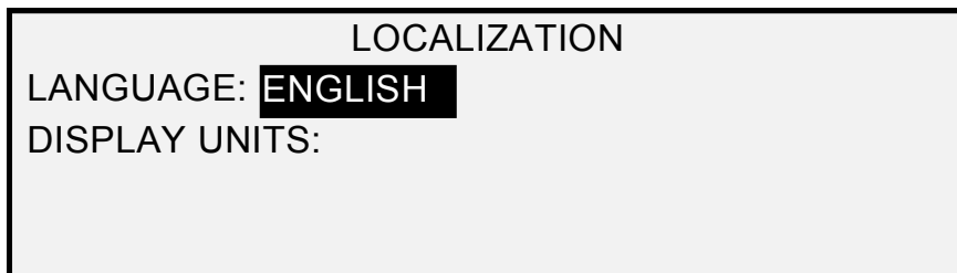
Localization Screen
