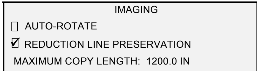
Imaging Screen
