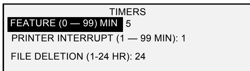
Timers Screen
