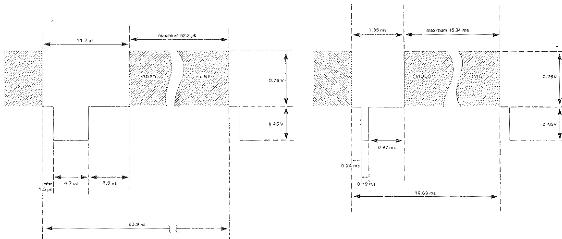
Horizontal Composite Waveform
