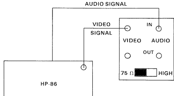
With an HP 82913A Video Monitor:
