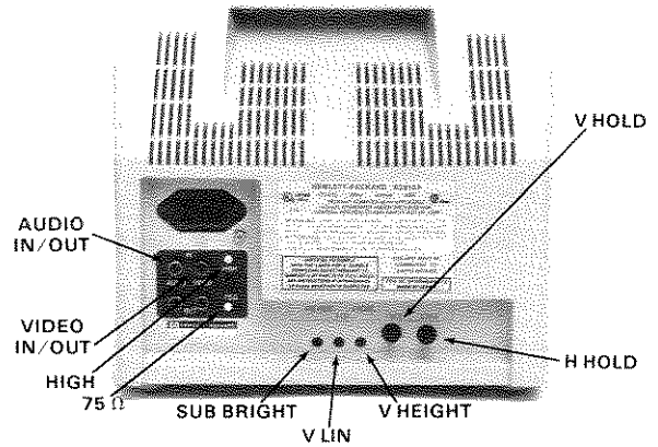
HP 82912A Video Monitor (9-inch)
