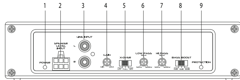
PA330 Input Plate
