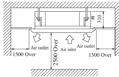
Installation space
