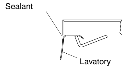
Undercounter Installation
