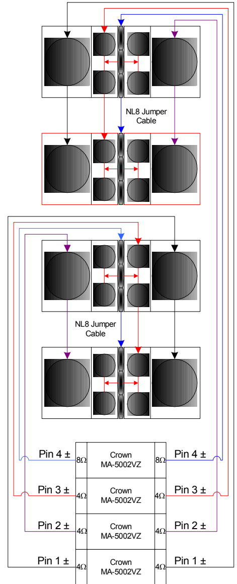
4 x Power Amplifiers (recommended)
