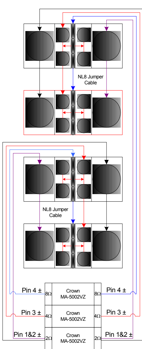
3 x Power Amplifiers (2Ω Load on LF Passband)
