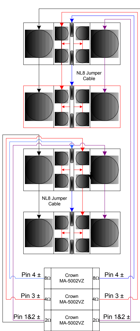
3 x Power Amplifiers (2Ω Load on LF Passband)
