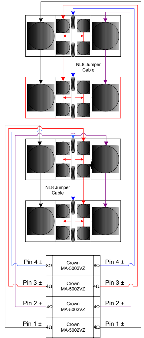
4 x Power Amplifiers (recommended)
