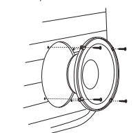
Figure 4. Mounting the P650c in a 165mm speaker location.
