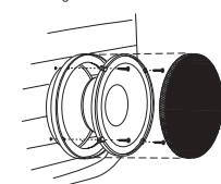
Figure 2. Mounting the P650c woofer with the grille.
