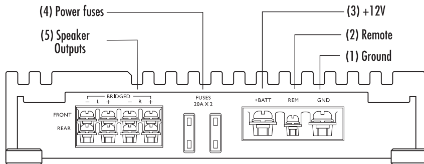
FIGURE 1—AMPLIFIER CONNECTIONS
