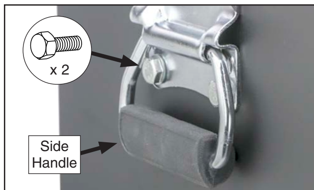
Figure 2. Side handle installed.
