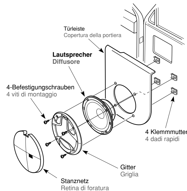
Abbildung 6 / Figura 6 (SRQ1720S)
