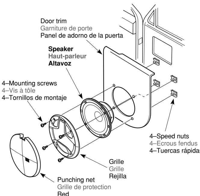
Figure 6 / Figure 6 / Figura 6 (SRQ1720S)
