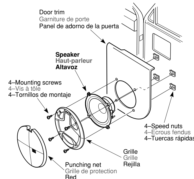
Figure 4 / Figure 4 / Figura 4 (SRQ1320S)
