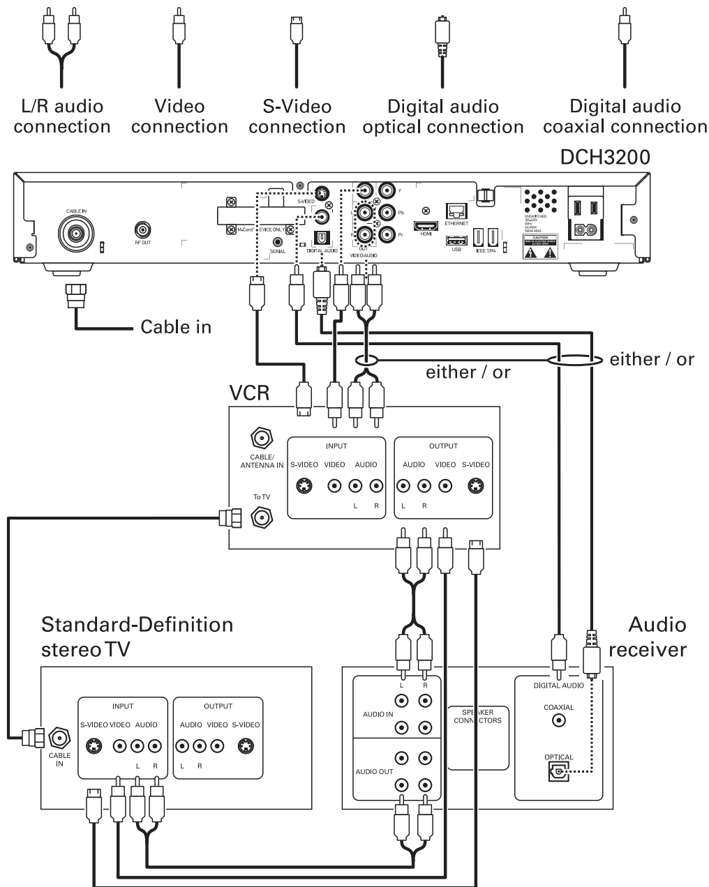
Figure 3-4 Cabling an audio receiver
