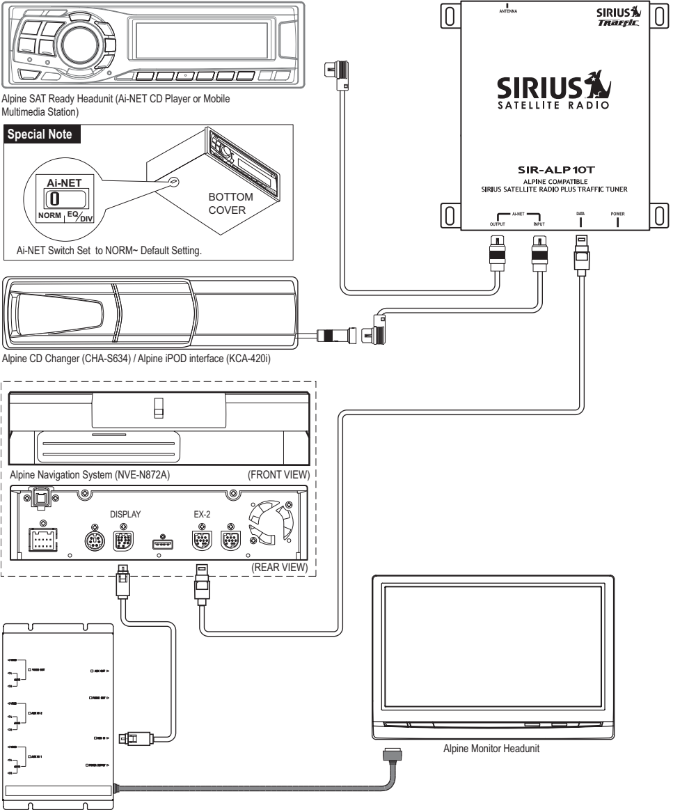
Alpine Monitor System (TME-M770 or TME-M710)
