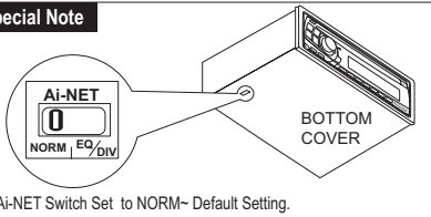
Alpine SAT Ready Headunit (Ai-NET CD Player or Mobile Multimedia Station)
