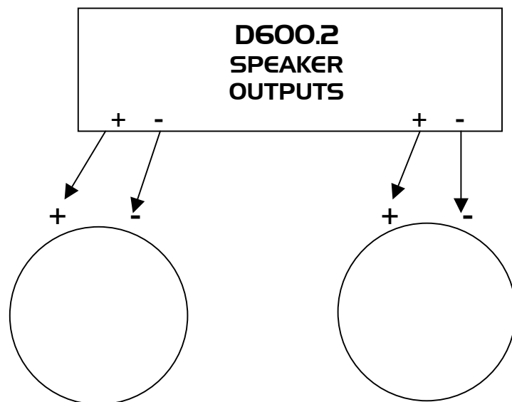
HOOKUP INTO TWO 4 OHM WOOFERS
