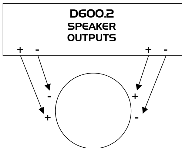
HOOKUP INTO ONE DUAL VOICE COIL (4 OHMS PER COIL) WOOFER
