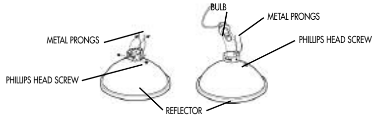
FIGURE 5 - BULB ASSEMBLY
