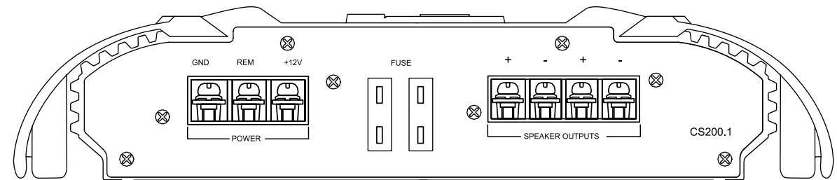
Figure 1. Terminal connection end plate.
