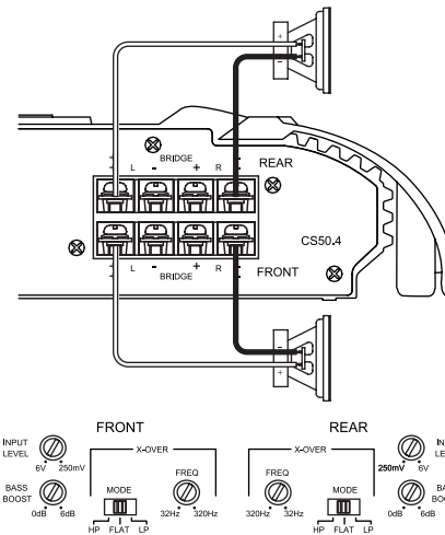
Figure 6. CS50.4 used in bridged 2-channel mode to drive a set of components or subwoofers. Set crossovers according to application.
