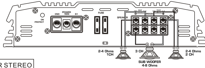
4 SPEAKER STEREO
