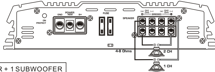
2 SPEAKER + 1 SUBWOOFER
