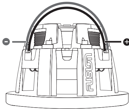
2 Ohm operation
