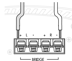
Figure 10: Bridged Single Woofer Connection
