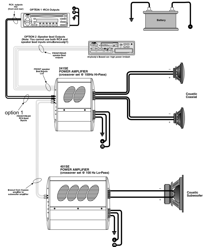
Figure 7. Typical Multi-amplifier system
