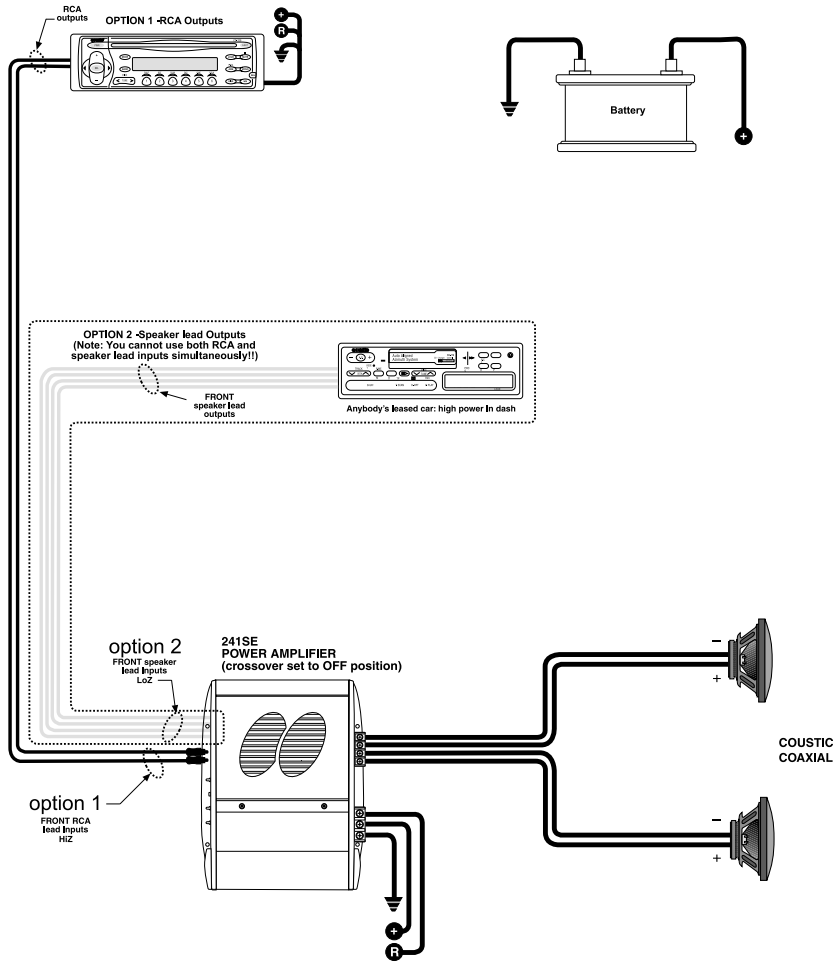
Figure 6. Typical System connection
