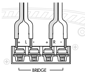
Figure 9: Stereo Connection
