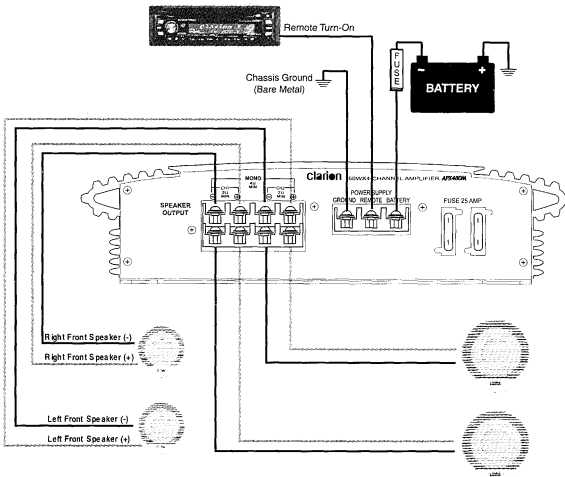
Figure 3 - Electrical connections
