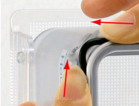
(Fig. 4) Stretch the O-ring
