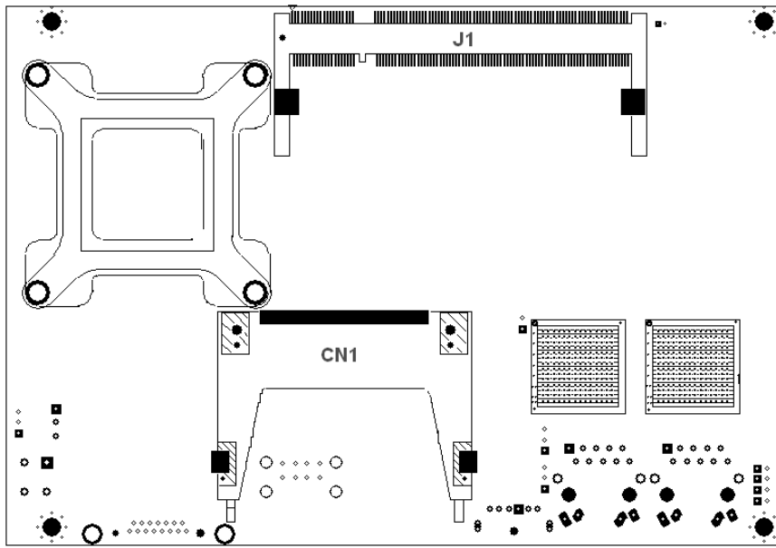
Bottom Placement
