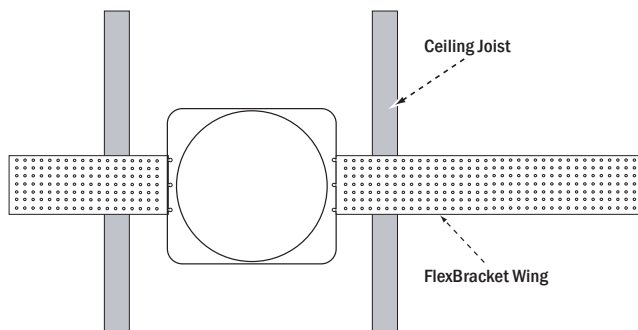
Illustration 2: Quintette FlexBracket Installation
