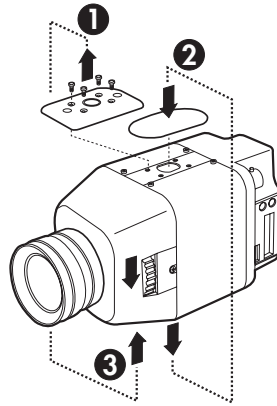
Figure 3. Camera Mounting
