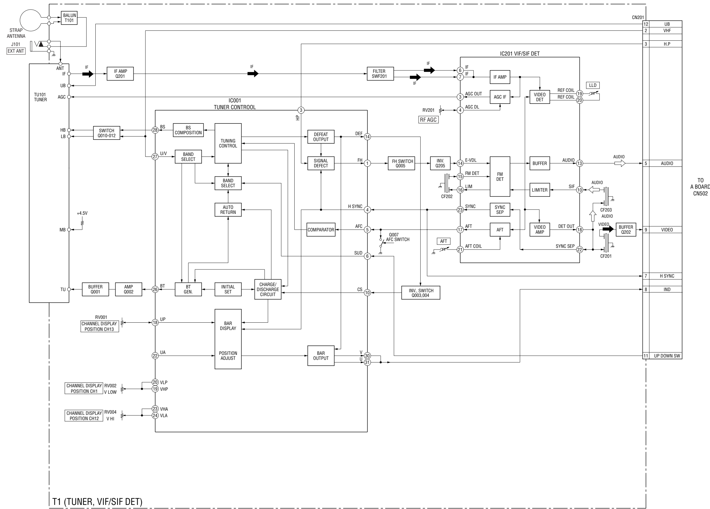
4-1. BLOCK DIAGRAM (1)
