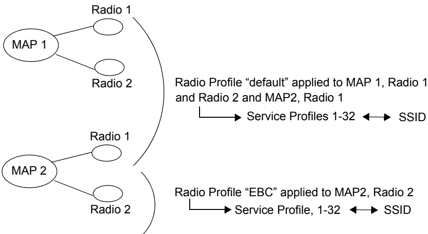
Figure 7 Radio and Service Profiles
