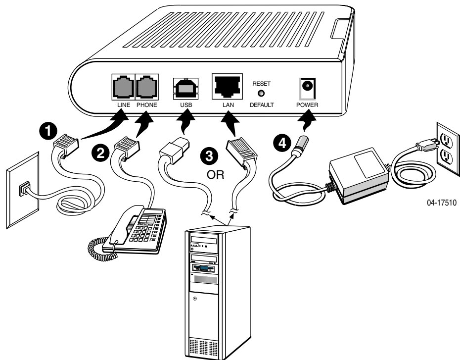
Figure 3: Hardware Installation
