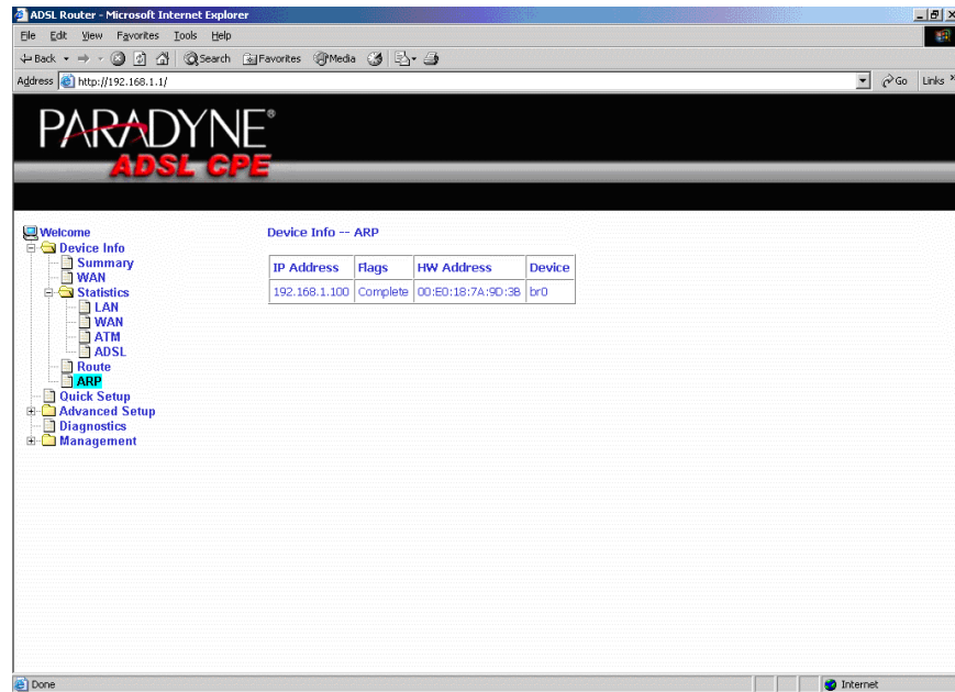
Figure 23: ARP Status
