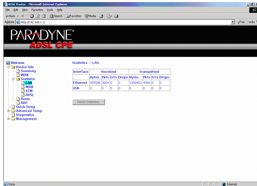
Figure 16: LAN Statistics
