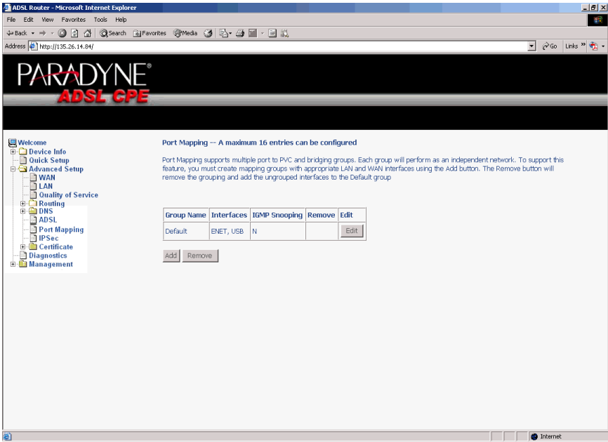
Figure 67: Port Mapping
