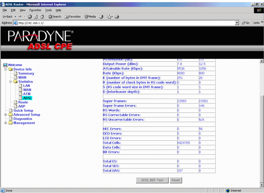
Figure 19: ADSL Status
