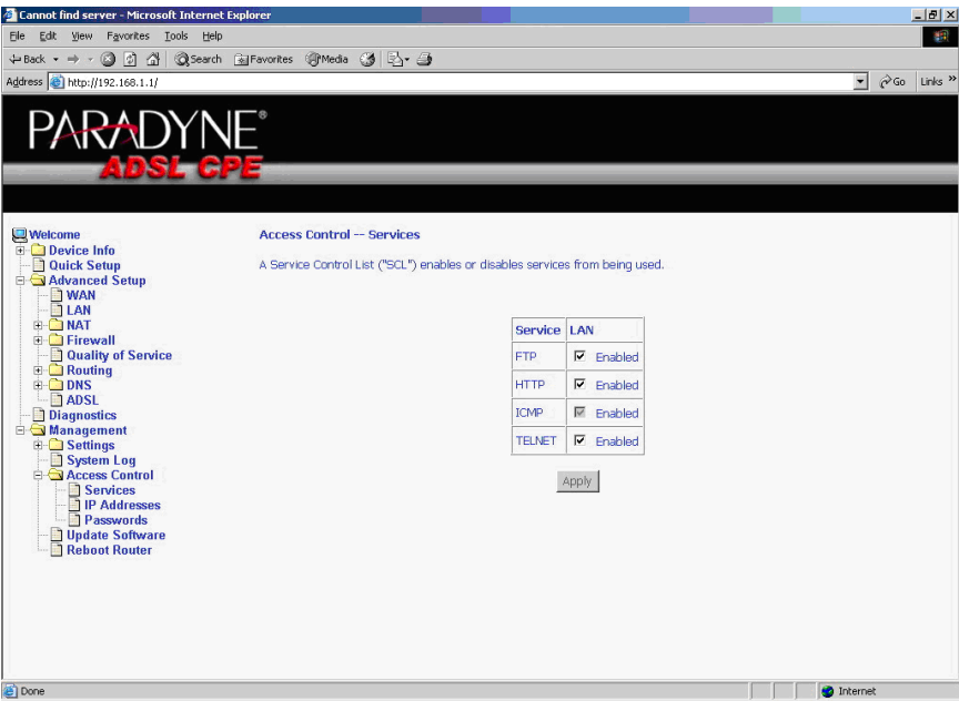
Figure 85: Services Setup
