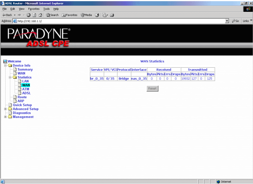
Figure 17: WAN Statistics
