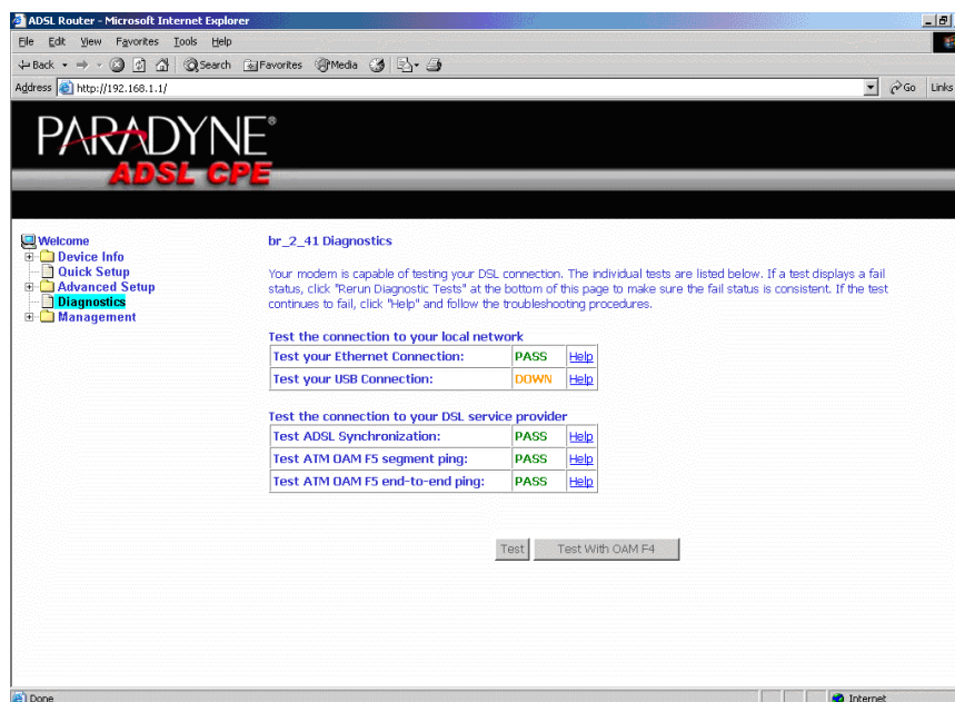
Figure 71: Diagnostics
