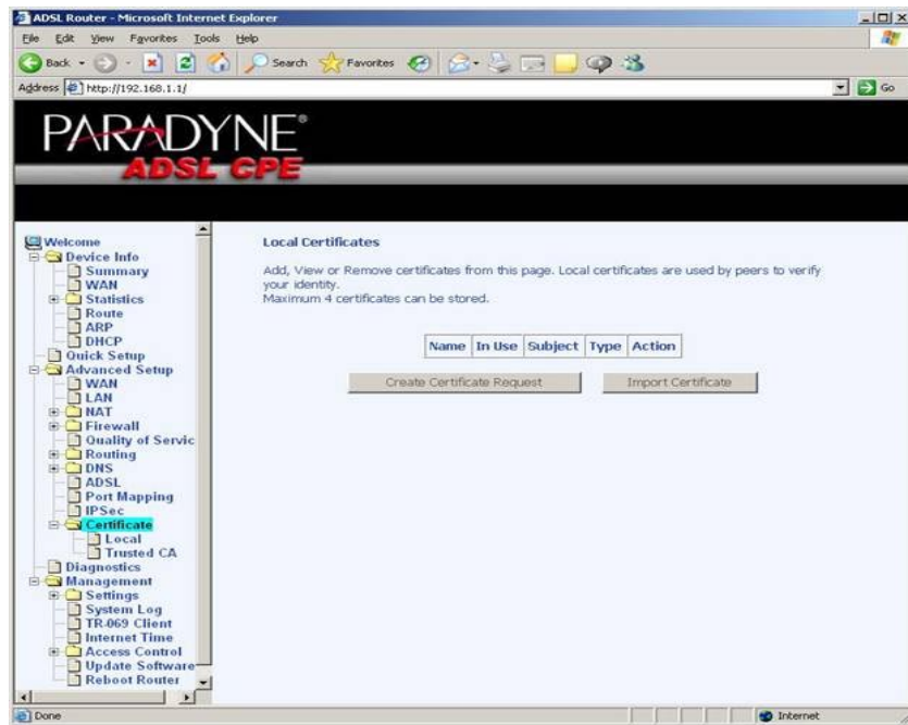
Figure 69: Certificate
