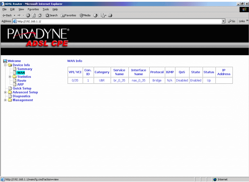
Figure 15: WAN Status
