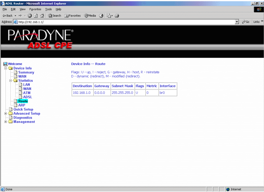
Figure 22: Route Information
