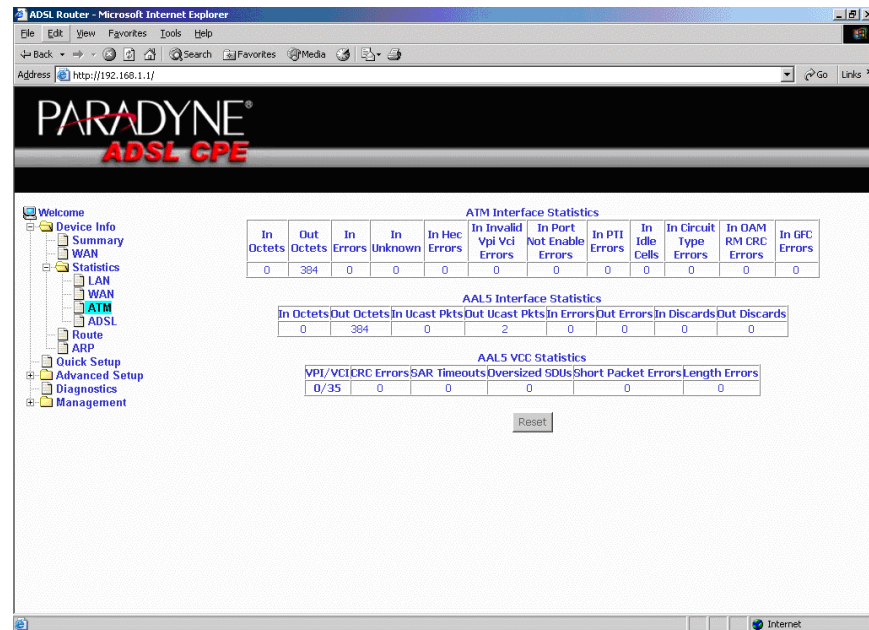
Figure 18: ATM Statistics
