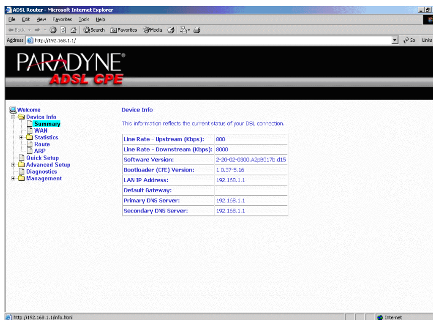
Figure 14: Status Summary
