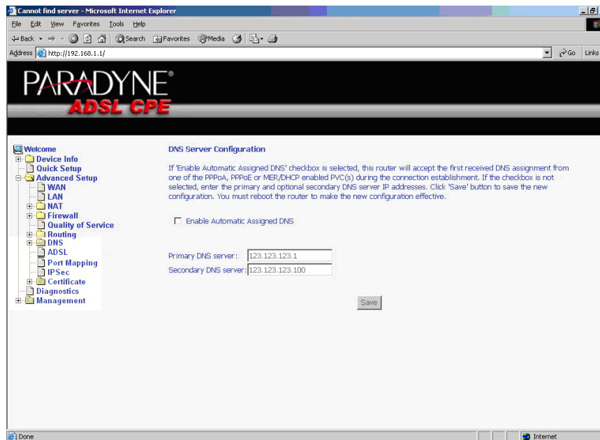
Figure 61: DNS Setup
