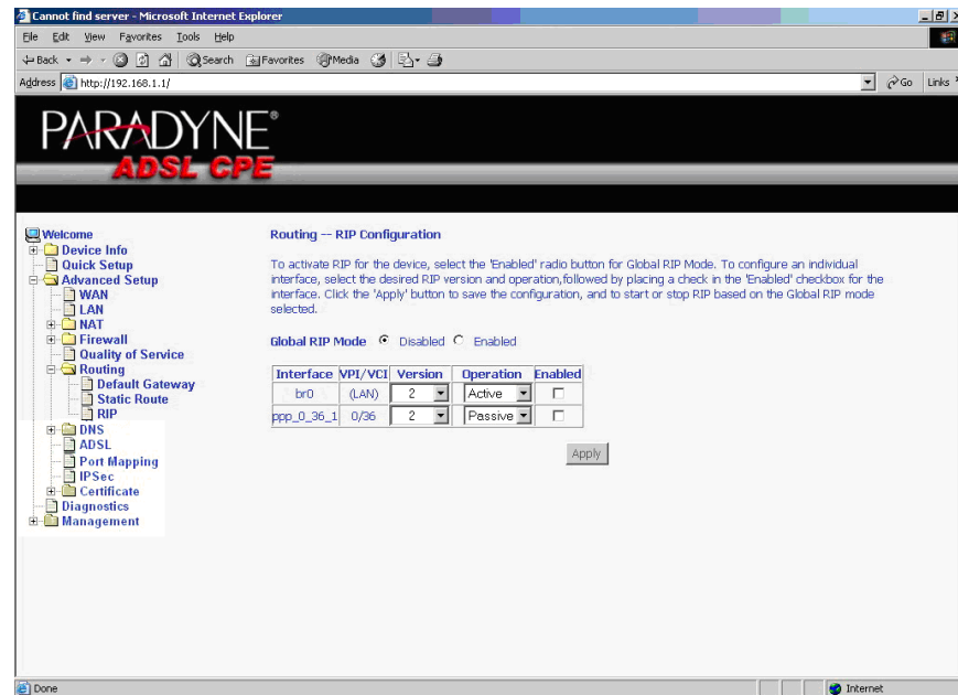
Figure 60: RIP Setup
