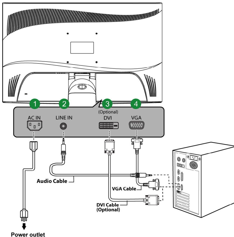
Figure.2. Connecting to a PC (HH241A/D)
