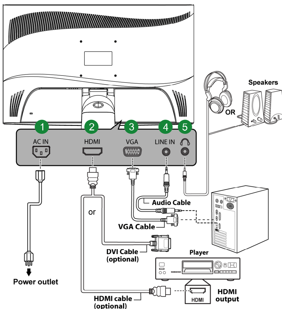
Figure.3. Connecting to a PC (HH241H)
