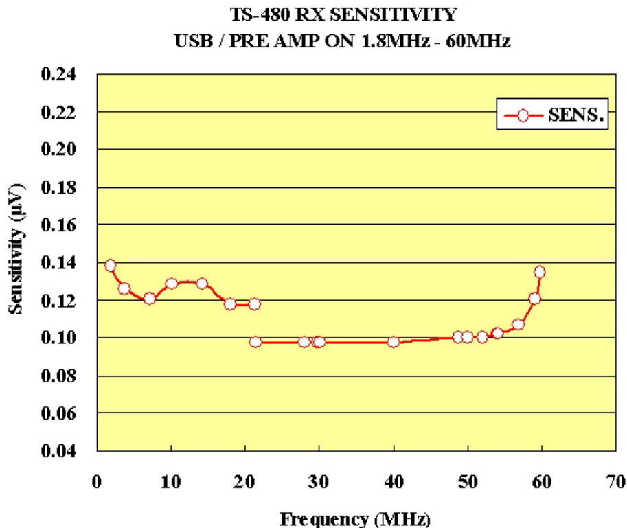
Fig. 9: RX sensitivity
