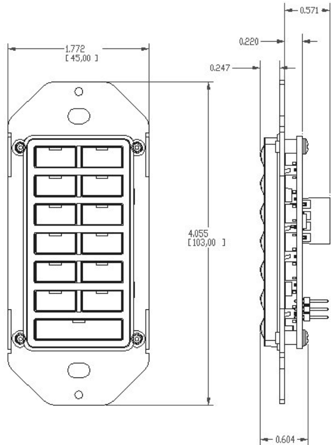
FIG. 6 Mounting Dimensions - MET-13
