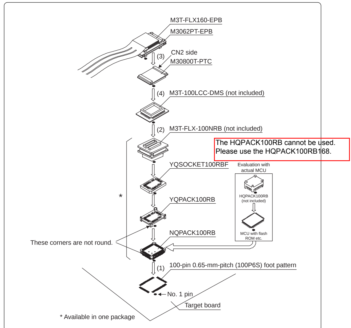
Figure 3.16 Connecting to a 100-pin 0.65-mm-pitch foot pattern (Part 3)
