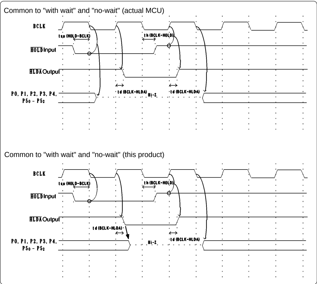
Figure 5.6 Timing requirements
