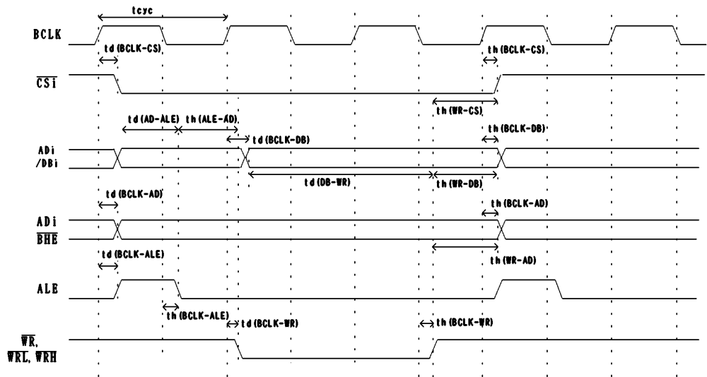
Figure 5.2 Memory expansion mode and microprocessor mode (2-wait, accessing external area, using multiplex bus)
