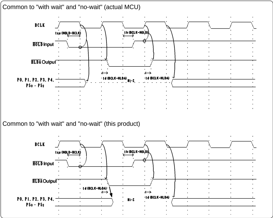
Figure 5.3 Timing requirements
