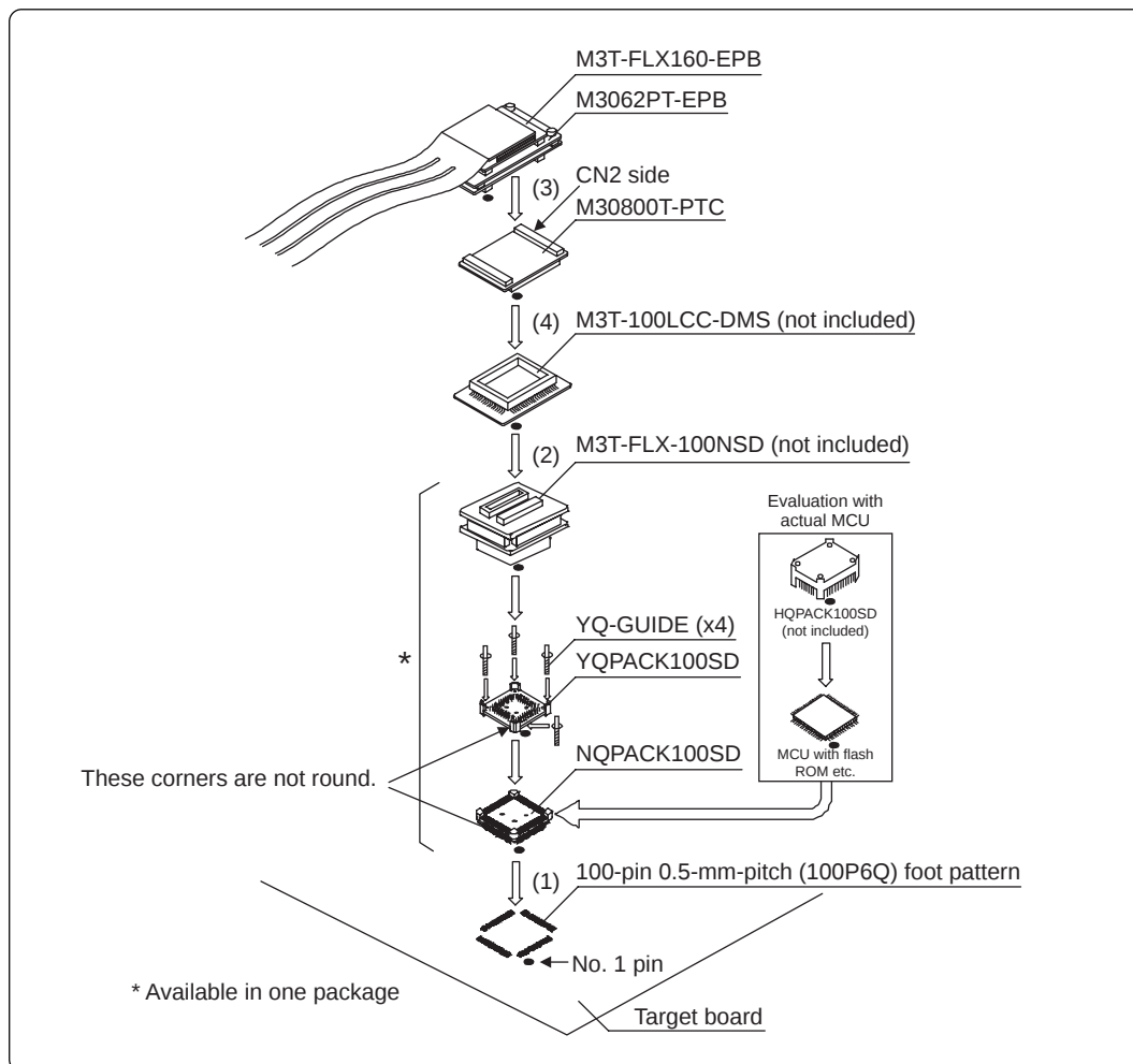
Figure 3.19 Connecting to a 100-pin 0.5-mm-pitch foot pattern (Part 3)
