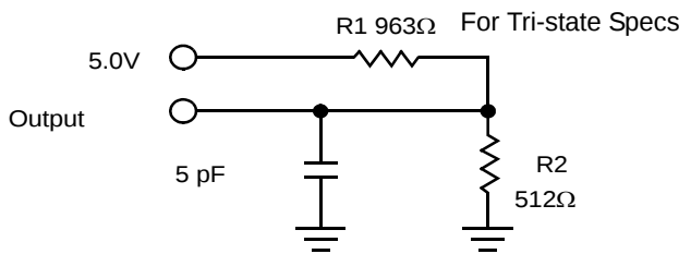
Figure 7. AC Test Loads
