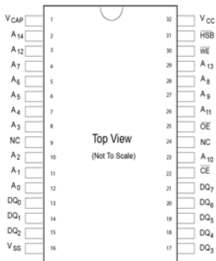
Figure 1. Pin Diagram: 32-Pin DIP
