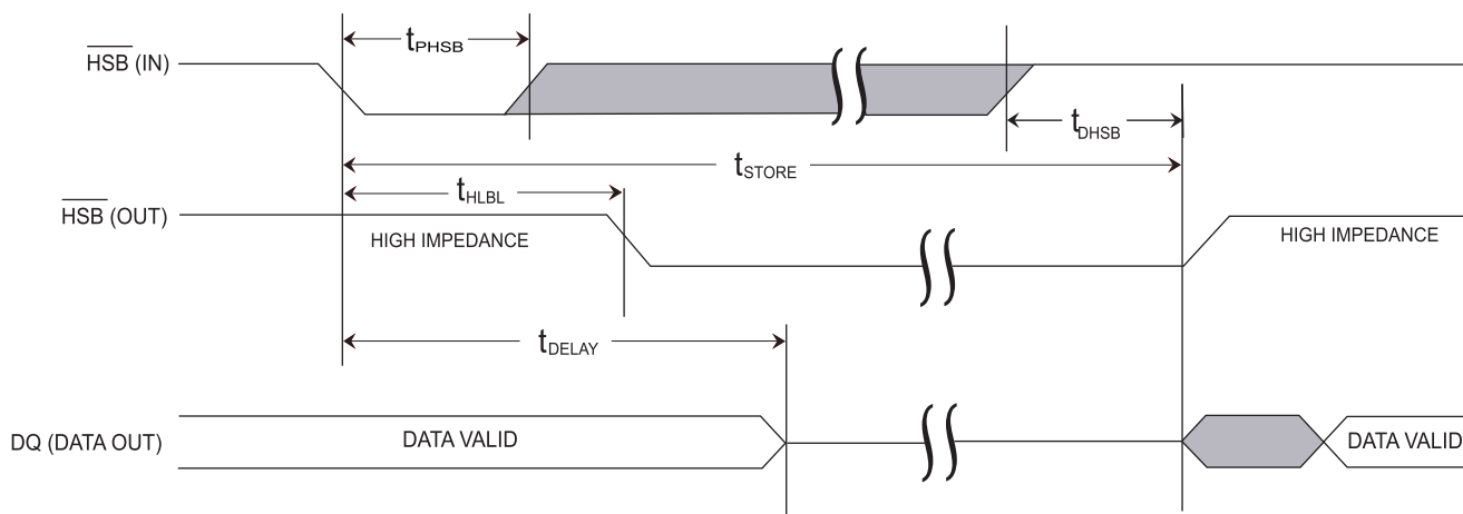
Figure 14. Hardware STORE Cycle
