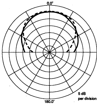
Figure 3. POLAR PATTERNS
