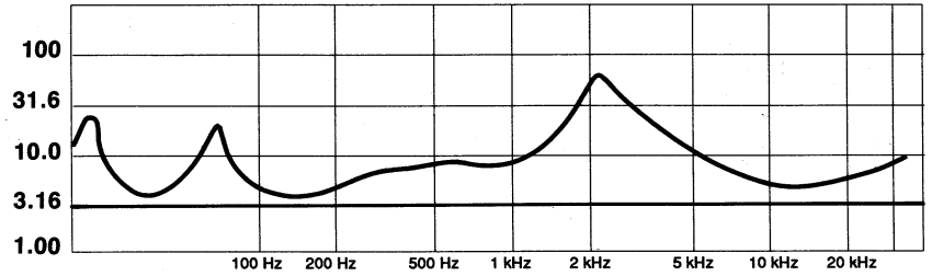
Figure 2. IMPEDANCE
