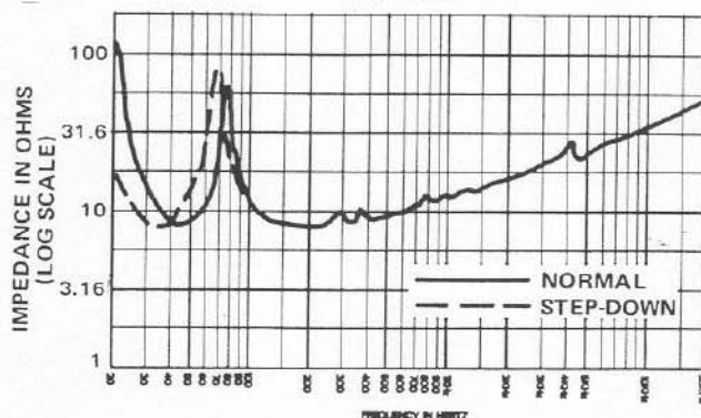
FIGURE 3B — Input Impedance vs. Frequency 7.1-Ft 3 (TL505) Enclosure
