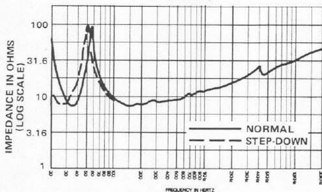
FIGURE 3A — Input Impedance vs. Frequency 13-Ft 3 Enclosure (TL405)
