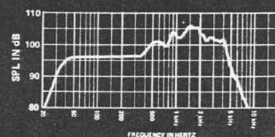
FIGURE 1 — Axial Frequency Response 1 Watt/1 Meter
