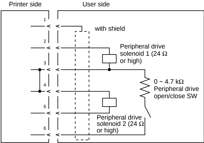
<Cable Connection 1>
