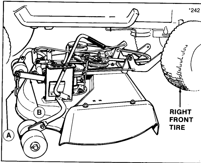
Figure 1. Installing 36" Mower
