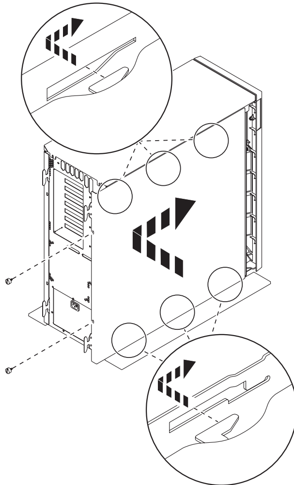
Figure 8. Install system unit side cover
