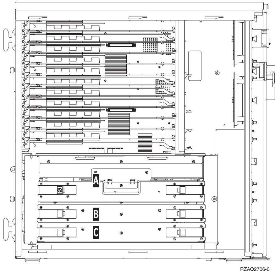
Figure 3. Location of Card Assembly 2884 in 820 Unit
