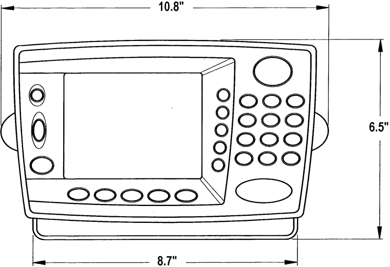
Figure 13—941X Dimensions
