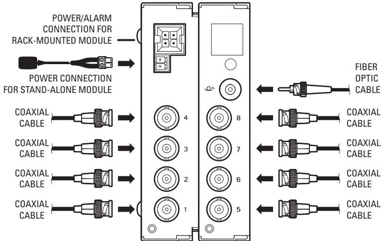
Figure 7. FT8308 Transmitter/FR8308 Receiver Connections
