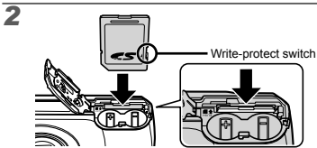
Battery/card compartment cover
