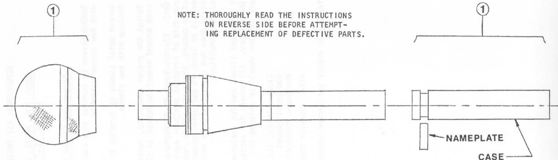
REPLACEMENT PARTS KITS FOR PL76, PL76A, PL77, PL77A MICROPHONE
