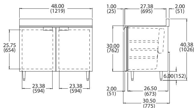
UR-48-SBS FRONT VIEW
