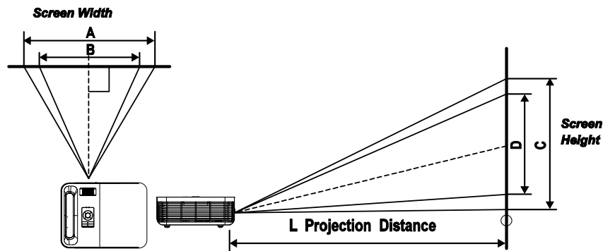
Projection distance and size table (0.55 inches)
