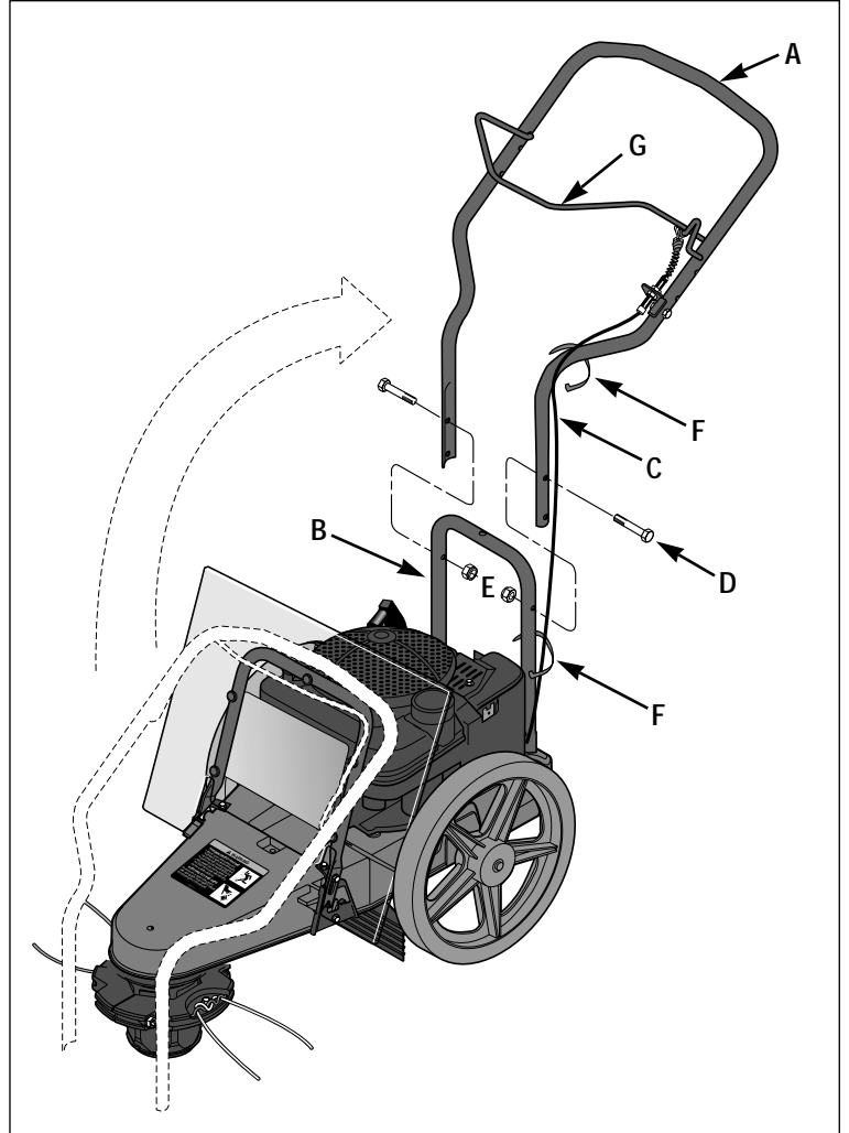
Figure 2-2: Handlebar installation.
