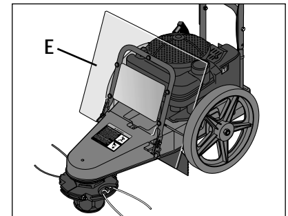
Figure 3-1A: Debris shield in operating position.
