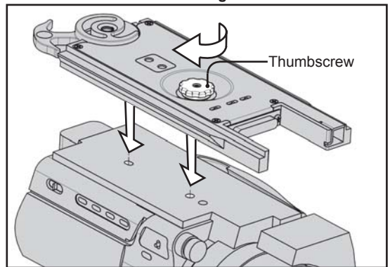
Connecting the HDR-FX1
