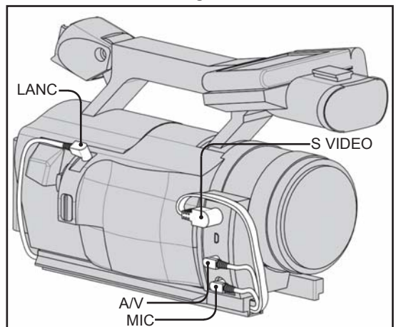
Connecting the HDR-FX1
