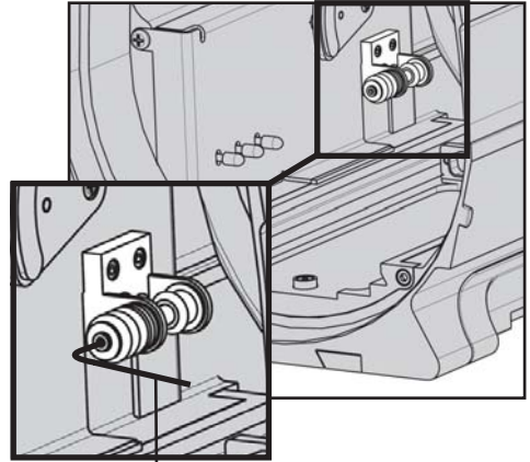
Allen Key (supplied)
