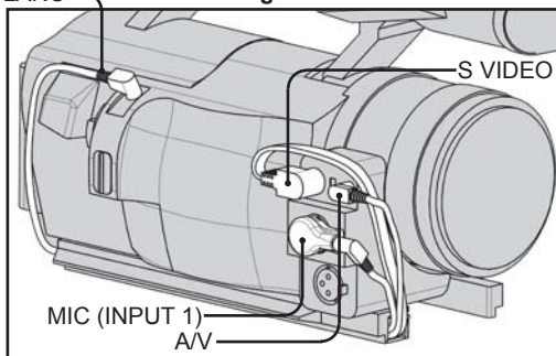
Connecting the HVR-Z1
