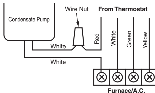
Figure 1: Low Voltage Auxiliary Safety Switch connection for Furnace/AC shutdown installation.
