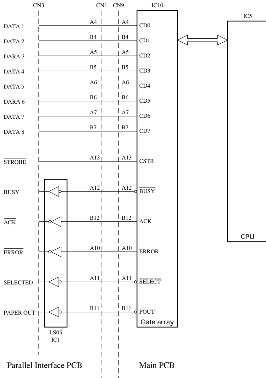
Fig. 2-4 Parallel Interface
