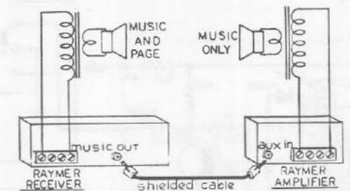
MUSIC OUTPUT OF RECEIVER USED TO DRIVE EXTERNAL AMPLIFIER FOR SIMULTANEOUS MUSIC ONLY OPERATION.
