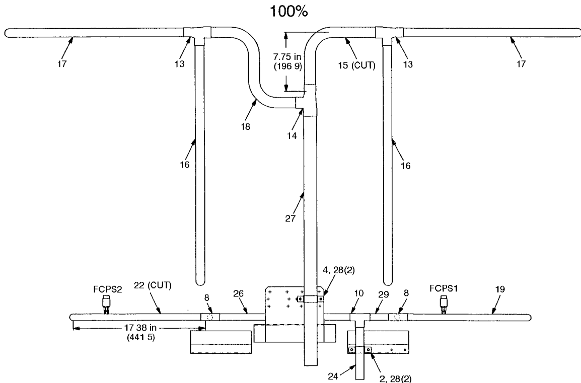
Fig. 14 — 100% Coil Circuiting; 054 and 064 Units
