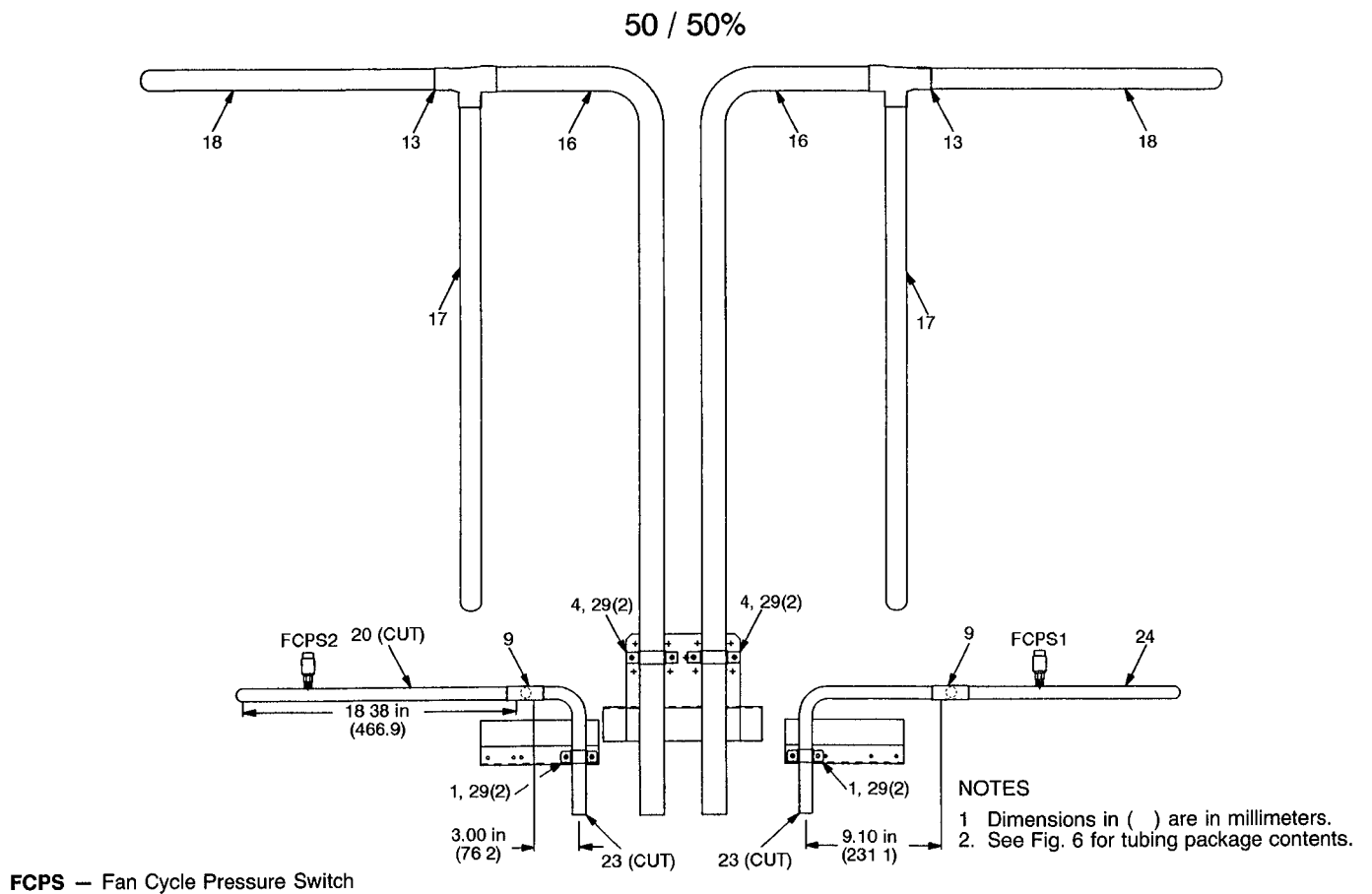
Fig. 24 — 50/50% Coil Circuiting; 084 Units
