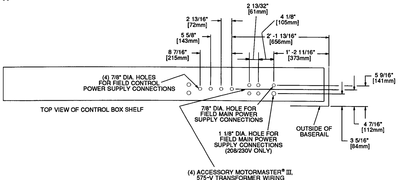
Fig. 30 — Power Wiring Access Holes; 054-094 Units
