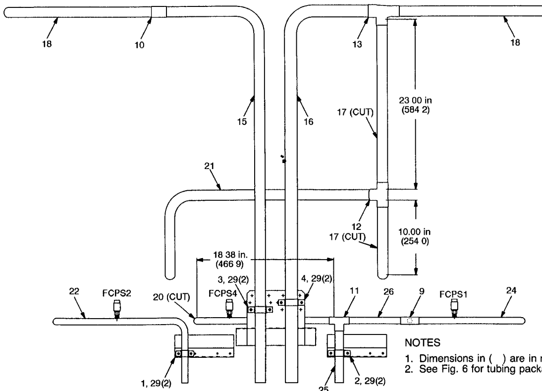
Fig. 22 — 68/32% Coil Circuiting; 074 Units
