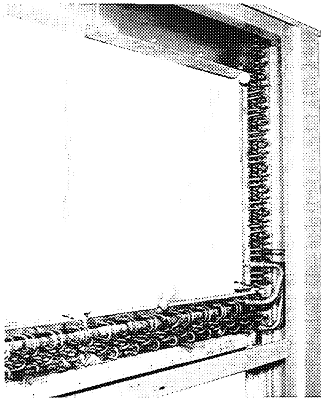
Fig. 12 — Typical Factory-Supplied Coil Circuiting, 09DK054-094 Units (084 Shown)
