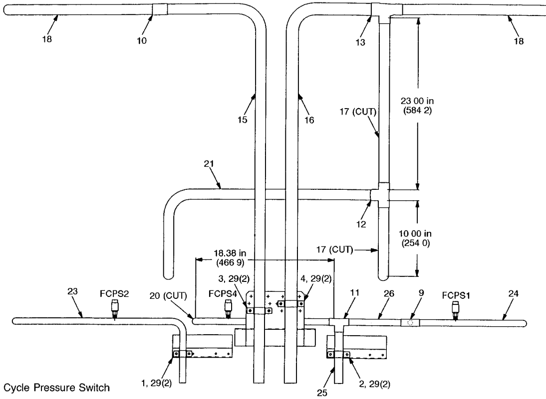
Fig. 25 — 67/33% Coil Circuiting; 084 Units
