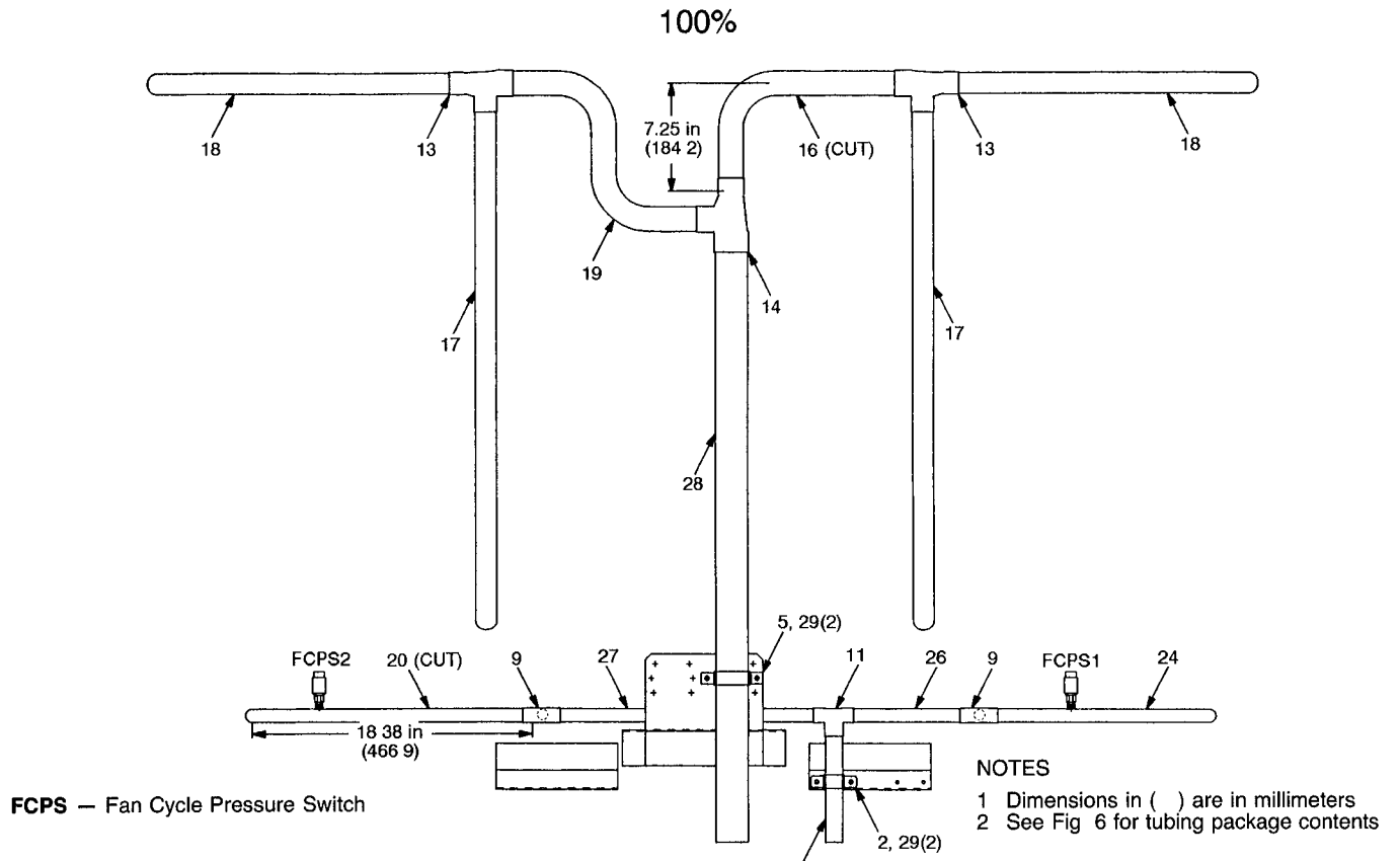
Fig. 23 — 100% Coil Circuiting; 084 Units
