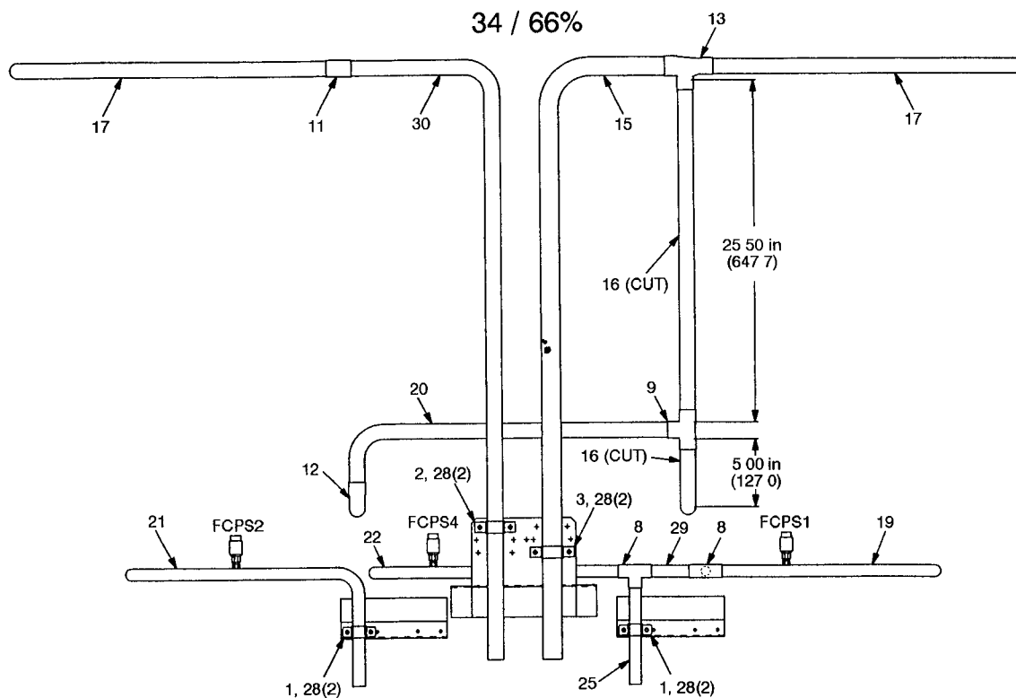
Fig. 17 — 50/50% Coil Circuiting; 054 and 064 Units
