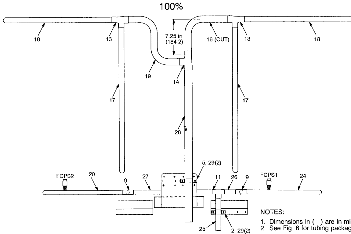
Fig. 19 – 100% Coil Circuiting; 074 Units
