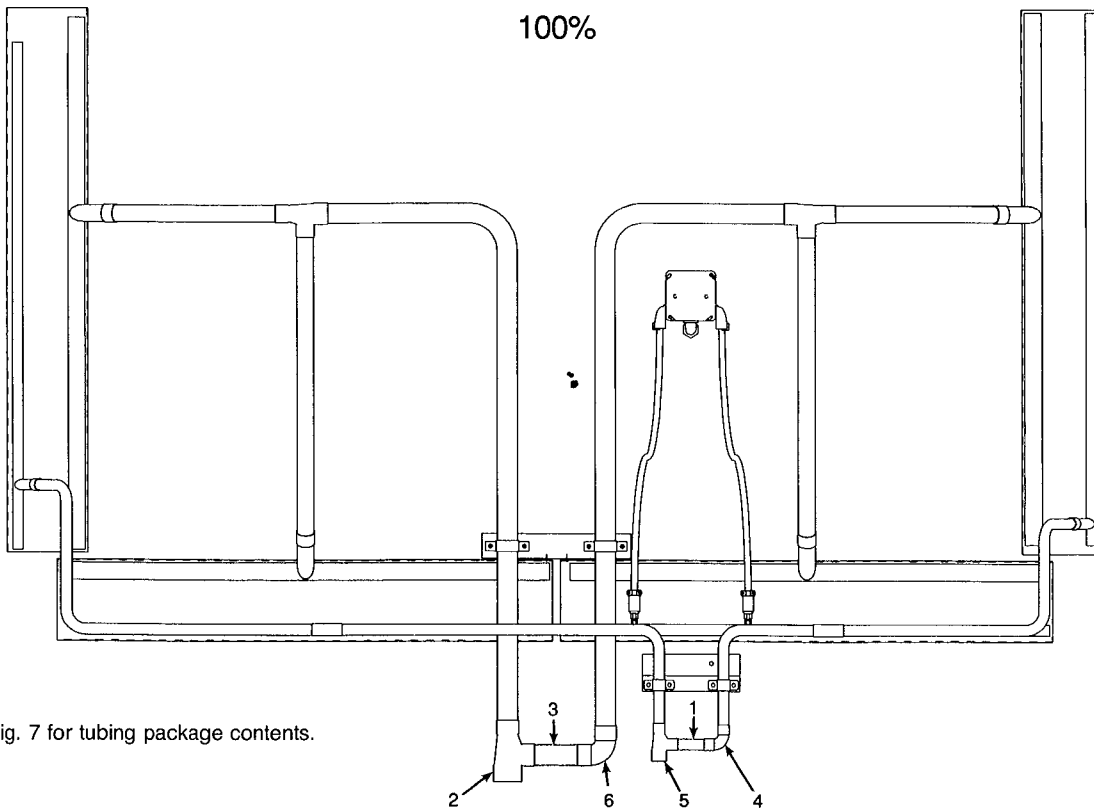
Fig. 26 — 100% Coil Circuiting; 094 Units
