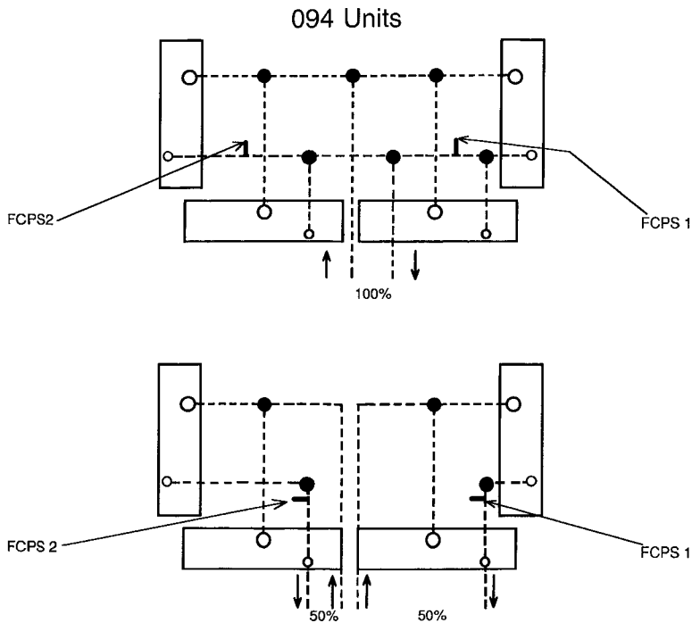
Fig. 9 – Typical Field Piping Arrangements (cont)
