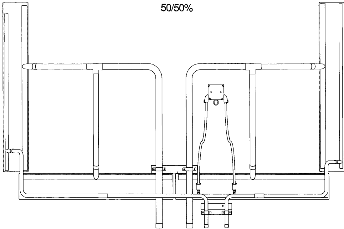
Fig. 27 – 50/50% Coil Circuiting; 094 Units
