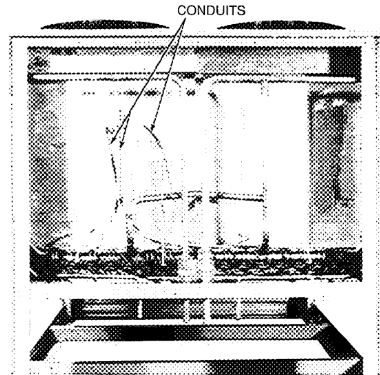
Fig. 13 — Typical Coil Circuiting for 09DK054-094 Units (67/33% Split Option; 084 Unit Shown)
