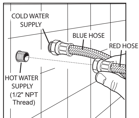
RED AND BLUE WATER SUPPLY LINES
